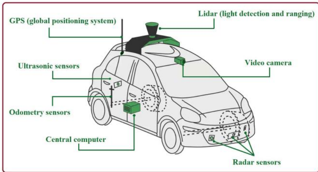
Figure 3.1.1 LiDAR equipped vehicle
